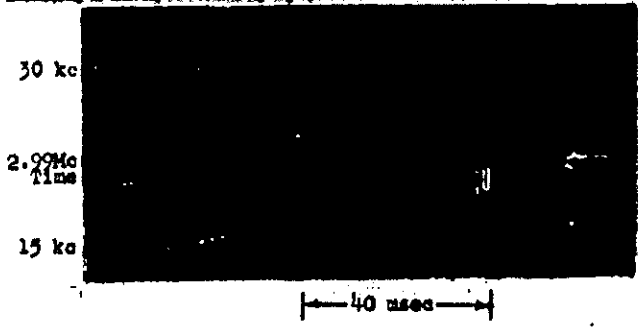
Fig. 3.75 Narrow-band responses Shot No. 6 1000 km from ground zero
